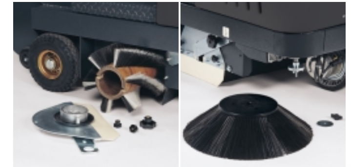
Self-adjusting central broom for proper contact with the ground. Flexible side brush to protect against bumps. Both of them can be removed and replaced without the help of any tools.
